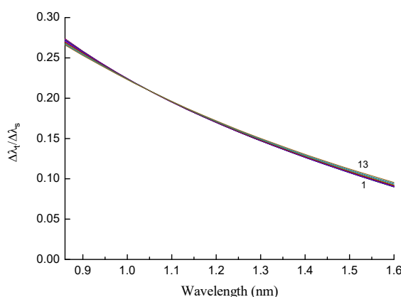
Figure 15. Temperature dependence of figure of merit for a 20 mm grating in B/Ge#1 fiber for modes LP_{11} – LP_{1,13} and \Delta T = 10\text{ K} (290–300 K).
