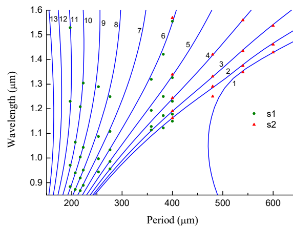
Figure 5. Resonance wavelengths of LPFGs vs. grating period for different LP_{1j} cladding modes in the SMF-28 fiber.
