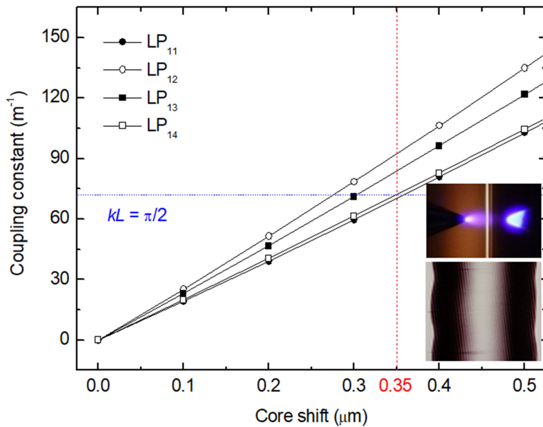
Figure 14. Coupling constant as a function of the core shift. Inset: Photograph of the microdeformation (fiber compressed on its length, showing two modulations separated by 540 μm) caused by the temperature gradient of the DC arc discharge. Adapted with permission from ref. [103]. © 2007 The Optical Society.
