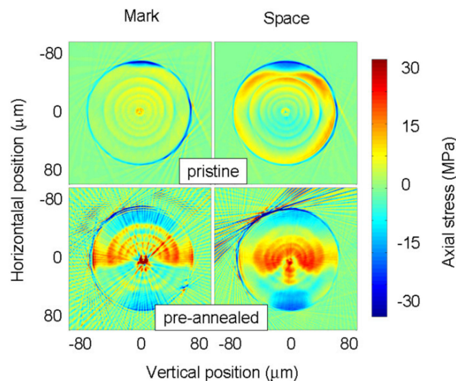
Figure 12. Comparison of the tomographic stress profiles for LPFGs written in the pristine and pre-annealed fibre. Reprinted with permission from ref. [123]. © 2006 IEE.
