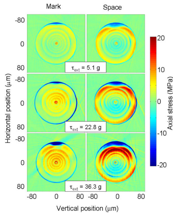
Figure 9. Tomographic stress profiles of the fiber drawn with the highest tension where LPFGs were induced using different pulling tensions. Reprinted with permission from ref. [118]. © 2005 IEEE.
