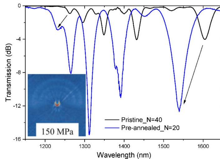
Figure 11. Spectra of gratings written in the pristine and pre-annealed fibre. Inset: Tomographic stress profile showing the “half-moon” stress induced in the core and inner cladding region of the pre-annealed by the arc discharge. Adapted with permission from ref. [123]. © 2006 IEE.
