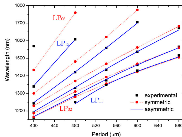
Figure 17. Dispersion curves for symmetric and asymmetric cladding modes. Adapted from [86].
