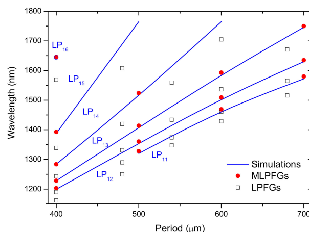
Figure 18. Dispersion curves corresponding to arc- and mechanically-induced gratings in the SMF28 fiber (simulations apply to MLPFGs). Reprinted with permission from ref. [131]. © 2008 Wiley Periodicals, Inc.
