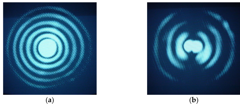
Figure 13. Intensity distribution in the near field for the (a) LP_{07} cladding mode of a 415 \mu\text{m} -LPFG written in the B/Ge fiber and (b) LP_{14} cladding mode of a 540 \mu\text{m} -LPFG written in the SMF28 fiber. Reprinted with permission from ref. [129]. © 2006 The Optical Society.
