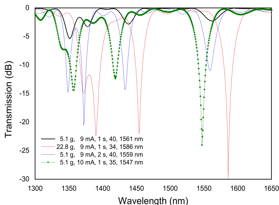
Figure 4. Influence of the fabrication parameters on LPFGs arc-induced in the SMF28 fiber. Adapted with permission from ref. [82]. © 2005 Taylor & Francis.
