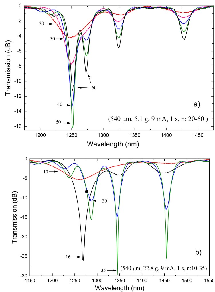
Figure 5. Influence of the fabrication parameters. Evolution of two LPFGs inscribed in the Sumitomo fiber (1.5 mol% GeO 2 ) using an external tension of (a) 5.1 g and (b) 22.8 g. Reprinted from [102].
