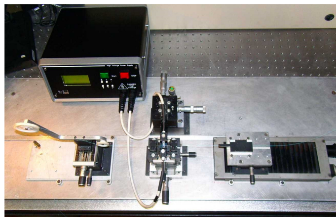
Figure 6. Experimental setup for LPFGs fabrication in the dispersion turning points. Reprinted with permission from ref. [98]. © 2016 IEEE.
