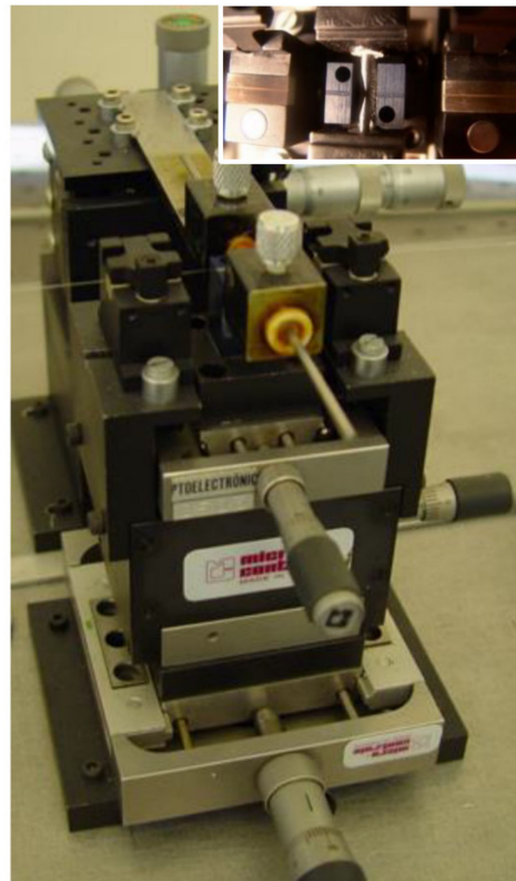
Figure 3. Central block showing the electrodes' support insulated with Teflon and the v-grooves mounted in different positioners. Inset: closer view of the electrodes and the v-grooves for fiber alignment.
