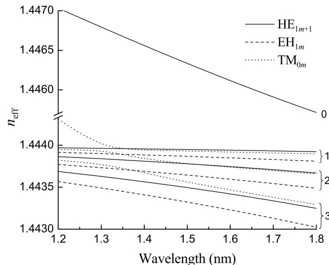
Figure 1. Dependences effective RI of the core mode and some cladding modes on wavelength. Numbering of the curves indicate the radial modal number m . Reprinted from [89].
