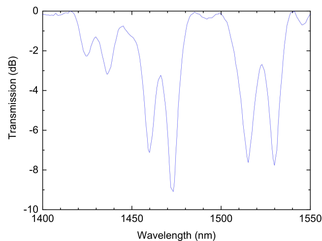
Figure 16. Gratings spectra containing a dual set of resonances inscribed simultaneously in the B/Ge codoped fiber. Reprinted with permission from ref. [130]. © 2007 The Optical Society.
