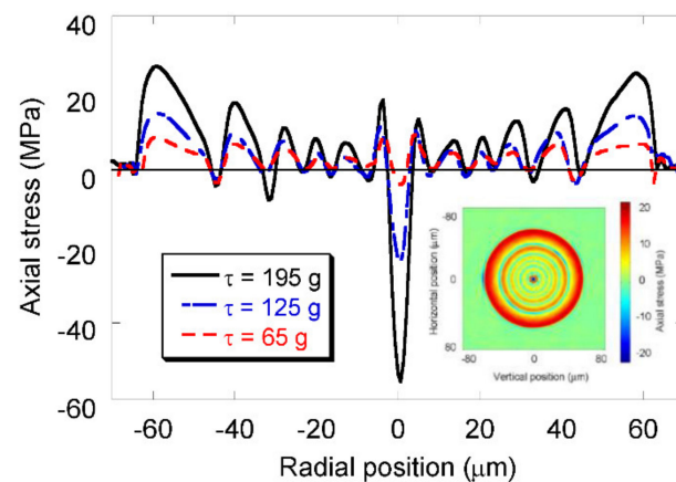
Figure 8. One-dimension tomographic stress profiles of the three fibers. Inset: 2D tomographic stress profile of the fiber drawn with a 125 g tension. Adapted with permission from ref. [118]. © 2005 IEEE.
