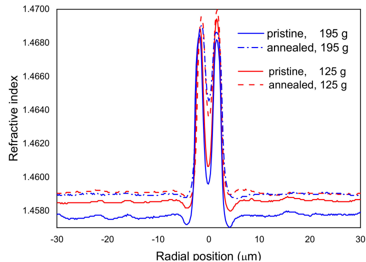
Figure 10. Refractive index profiles of the fibers drawn with 125 g and 195 g, before and after annealing. Reprinted with permission from ref. [123]. © 2006 IEE.
