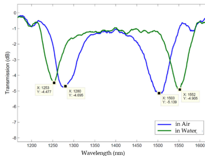
Figure 7. A 148 \mu\text{m} -LPFG in the DTP, arc-induced in a B/Ge co-doped fiber, immersed in air/water.
